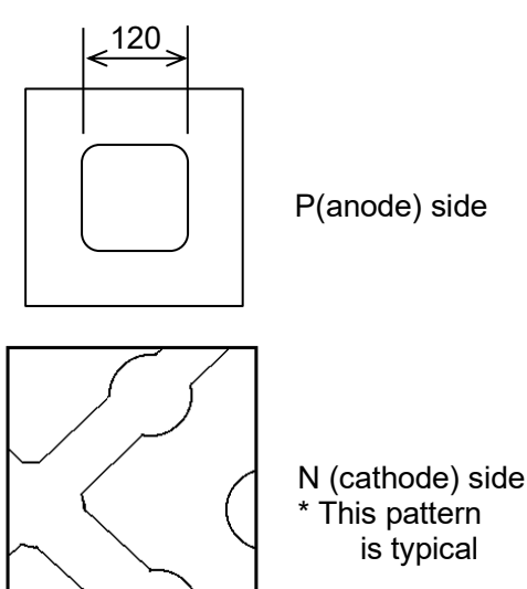
Fig.1 Electrode pattern
